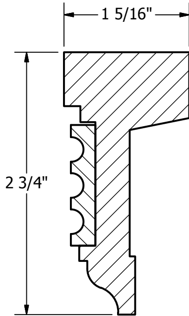
PROFILE SCALE 1 : 1
