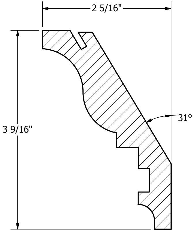
PROFILE SCALE 1 : 1
