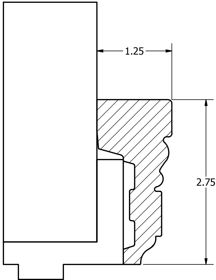
MG628H - PROFILE SCALE 1 : 1
