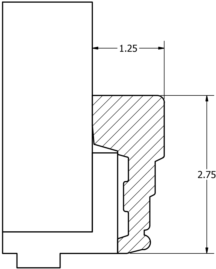
MG628C - PROFILE SCALE 1 : 1
