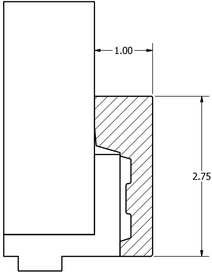
MG528P - PROFILE SCALE 1 : 1
