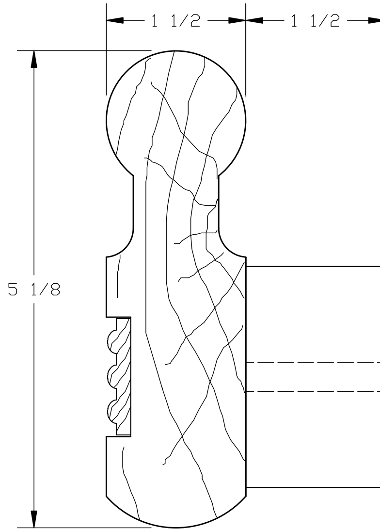
HR70 HANDRAIL WITH SR31B INSERT SELECTRIM CORP. 1-800-326-9734
