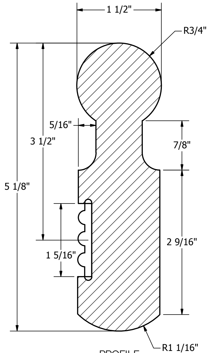
PROFILE SCALE 1 : 1
